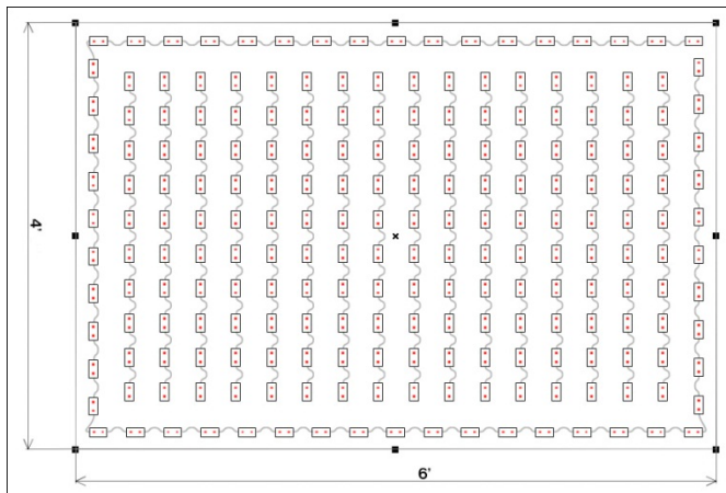
This is a 4' by 6' cabinet with a Hybrid population , 2" Edge Gap, and 4" Run Gap.
